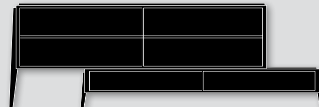
TV CABINET 341 2 doors, 2 drawers Dim : W. 200 x D.50 x H. 68
