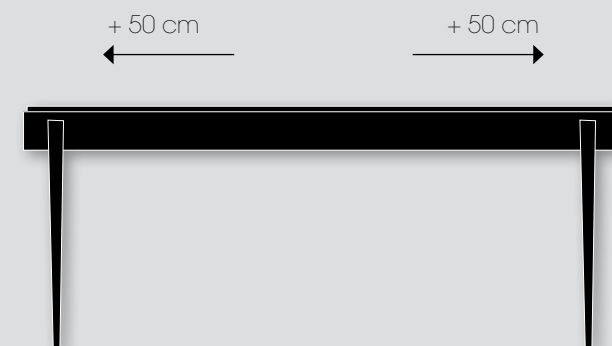
RECTANGULAR TABLE 350 2 extensions of 50 cm Dim : W. 140 x D. 110 x H. 77
